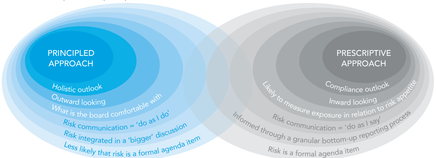
FIGURE 2.1: Principled–Prescriptive spectrum 1
